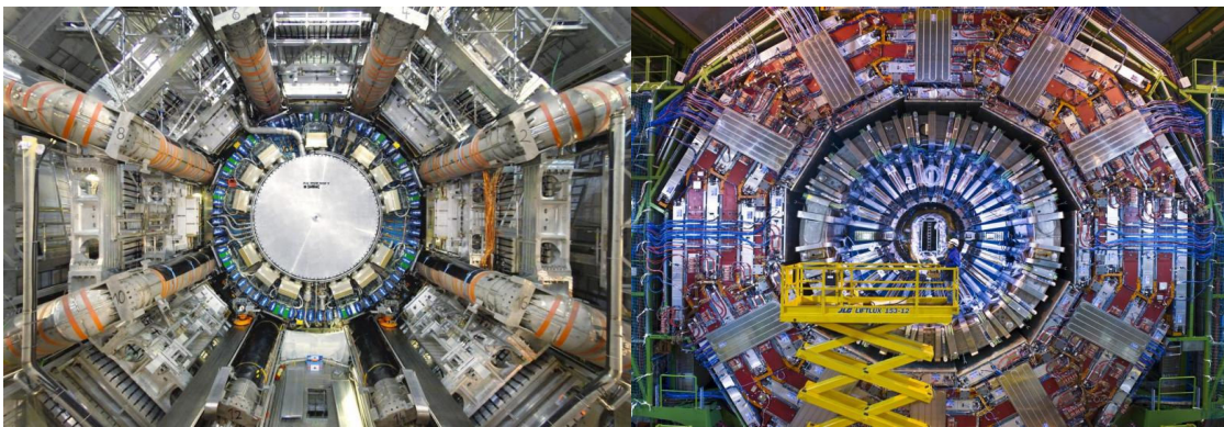
ATLAS CMS
